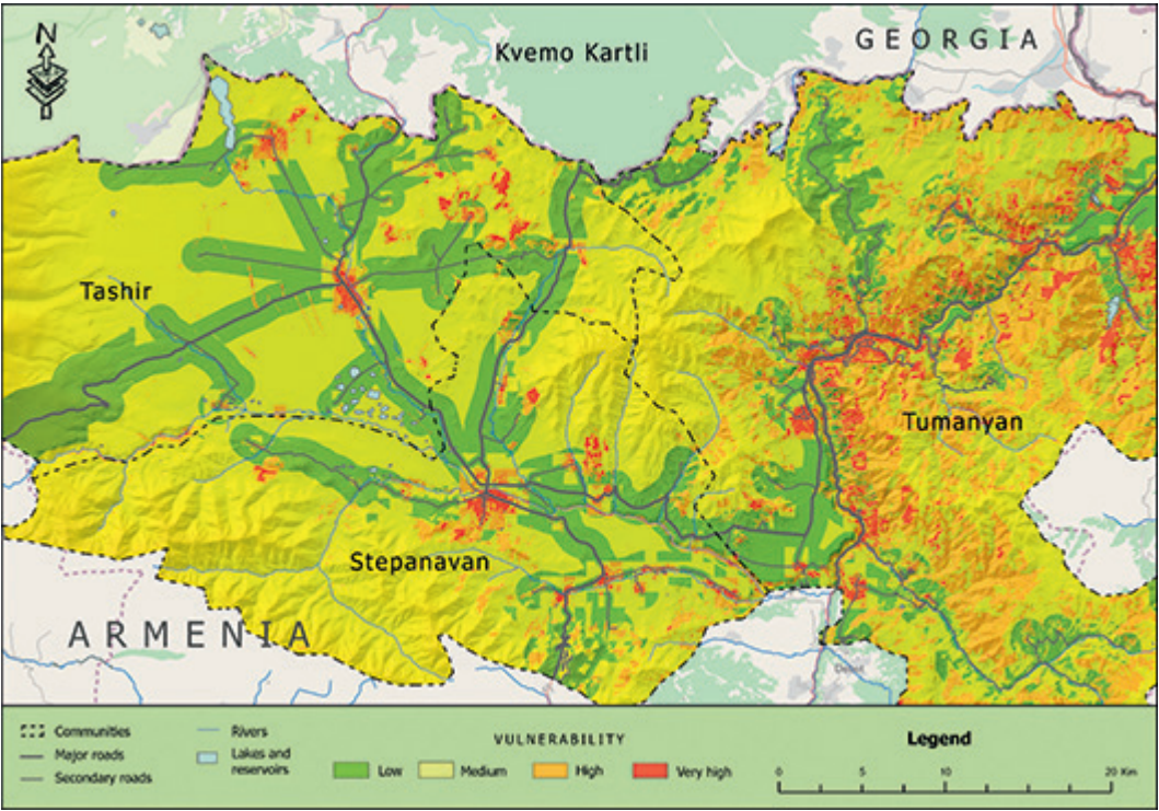
Map 7: Wildfire vulnerability map: Tashir, Stepanavan, and Tumanyan communities of Lori Marz, Armenia
