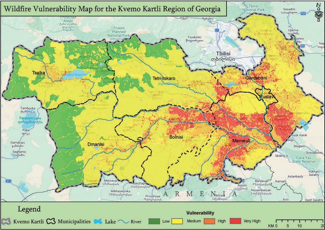
Map 6: Wildfire vulnerability map: Bolnisi, Dmanisi, Gardabani, Marneuli, Tetritskaro, Tsalka, and Rustavi municipalities of Shida Kartli, Georgia
