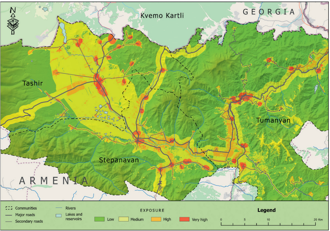
Map 5: Wildfire exposure map: Tashir, Stepanavan, and Tumanyan communities of Lori Marz, Armenia
