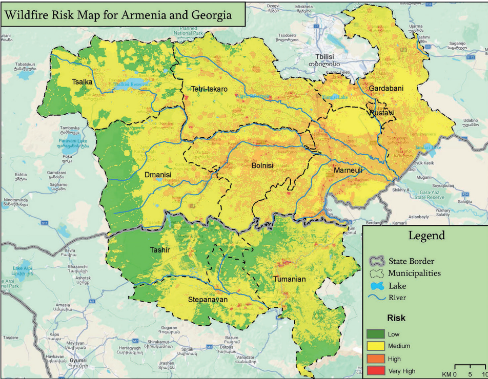
Map 10: Wildfire risk map of two bordering regions: Kvemo Kartli (Georgia) and Lori Marz (Armenia)
