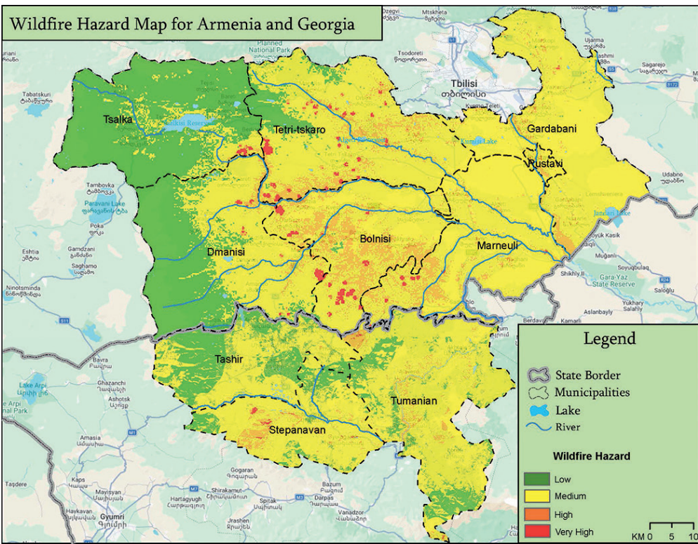
Map 3: Wildfire hazard map of two bordering regions: Kvemo Kartli (Georgia) and Lori Marz (Armenia)
